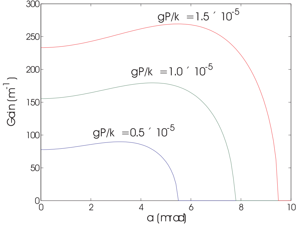
FIG. 2: Signal beam gain as a function of collision half-angle \alpha for \lambda = 700\text{nm} . Note that \Delta k = 2|\vec{k}_1|(1 - \cos \alpha) .
